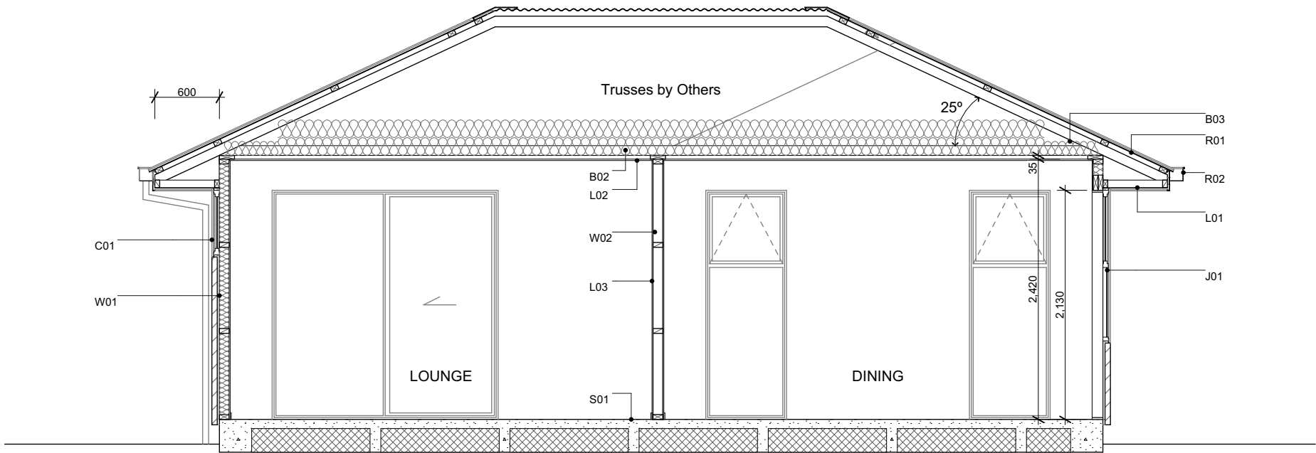
A Section A-A Scale 1:50
