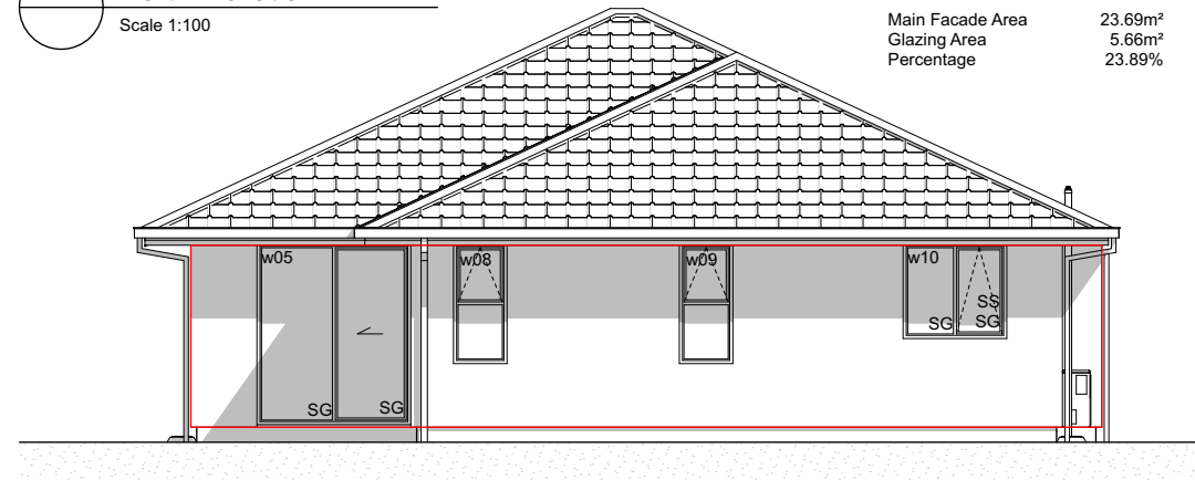
E-03 West Elevation Scale 1:100
