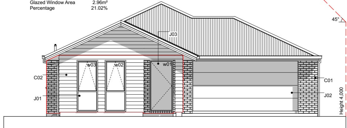
E-01 SouthWest Elevation Scale 1:100
